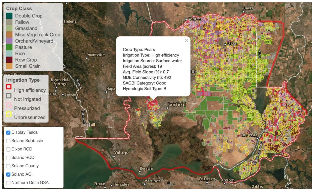
Figure 2. Crop classes and irrigation types for individual fields throughout the Solano AOI, as displayed in the web application. Polygon fill colors represent field crop types, and border colors represent irrigation types. Complete environmental and management data for a randomly selected field are shown in the data “pop-up” box.
