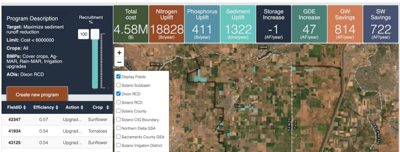
Figure 5. An example of outputs from the program planning feature of the web application, including the fields identified for implementation of specific practices to meet user-specified water resource objectives. Program costs and ancillary water resource impacts of the program are also shown.
