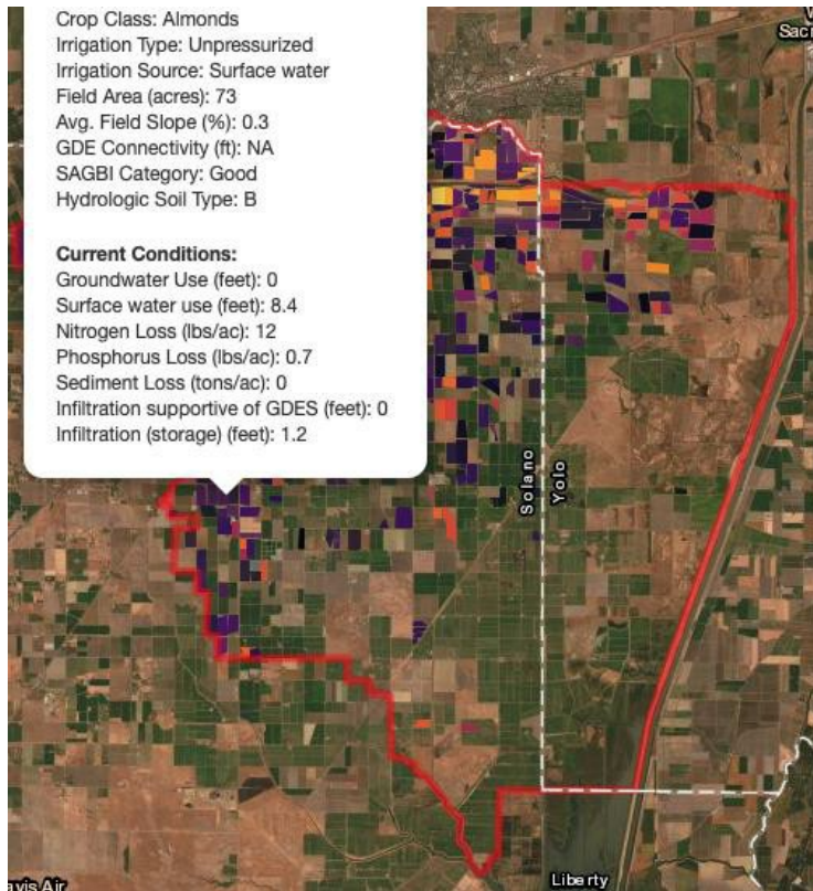
Figure 3. Current conditions within Dixon RCD. In this example view of the web application, the presence of field polygons indicates where cover cropping is likely feasible, and field color represents relative estimated nitrogen loss under current management. The pop-up displays the full suite of modeled values for a randomly-selected field under current management conditions.
